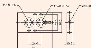
Single Acting Use Plate SN3000-Plate
